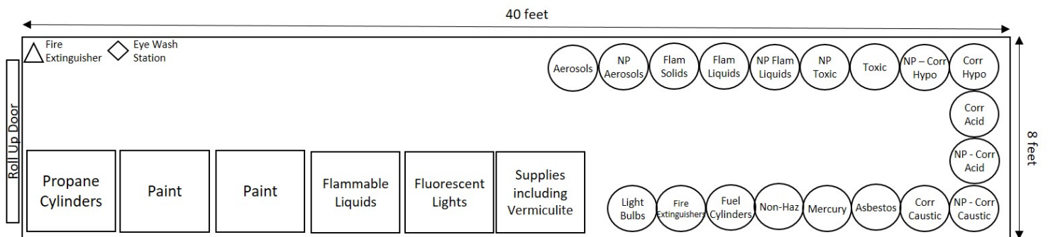
FIGURE 5: EXAMPLE OF STORAGE AREA LAYOUT FOR HHW SEACAN
